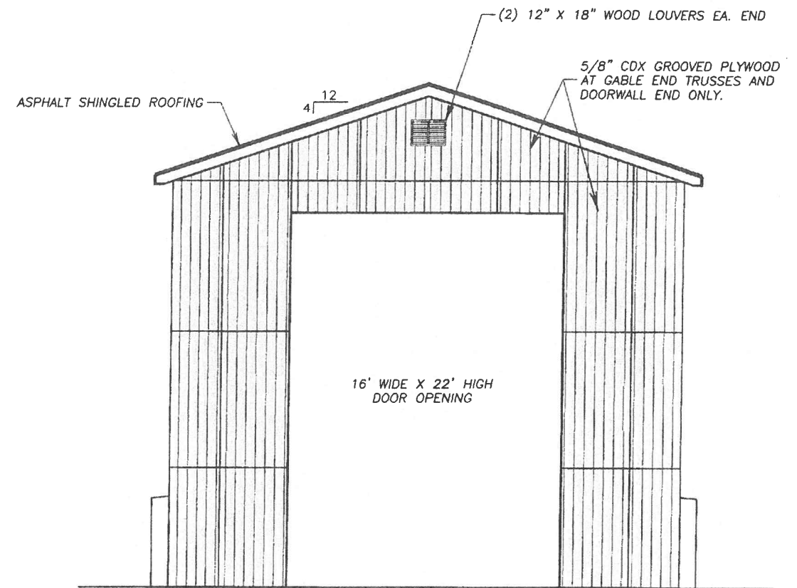
DOORWALL VIEWING FROM OUTSIDE STRUCTURE
