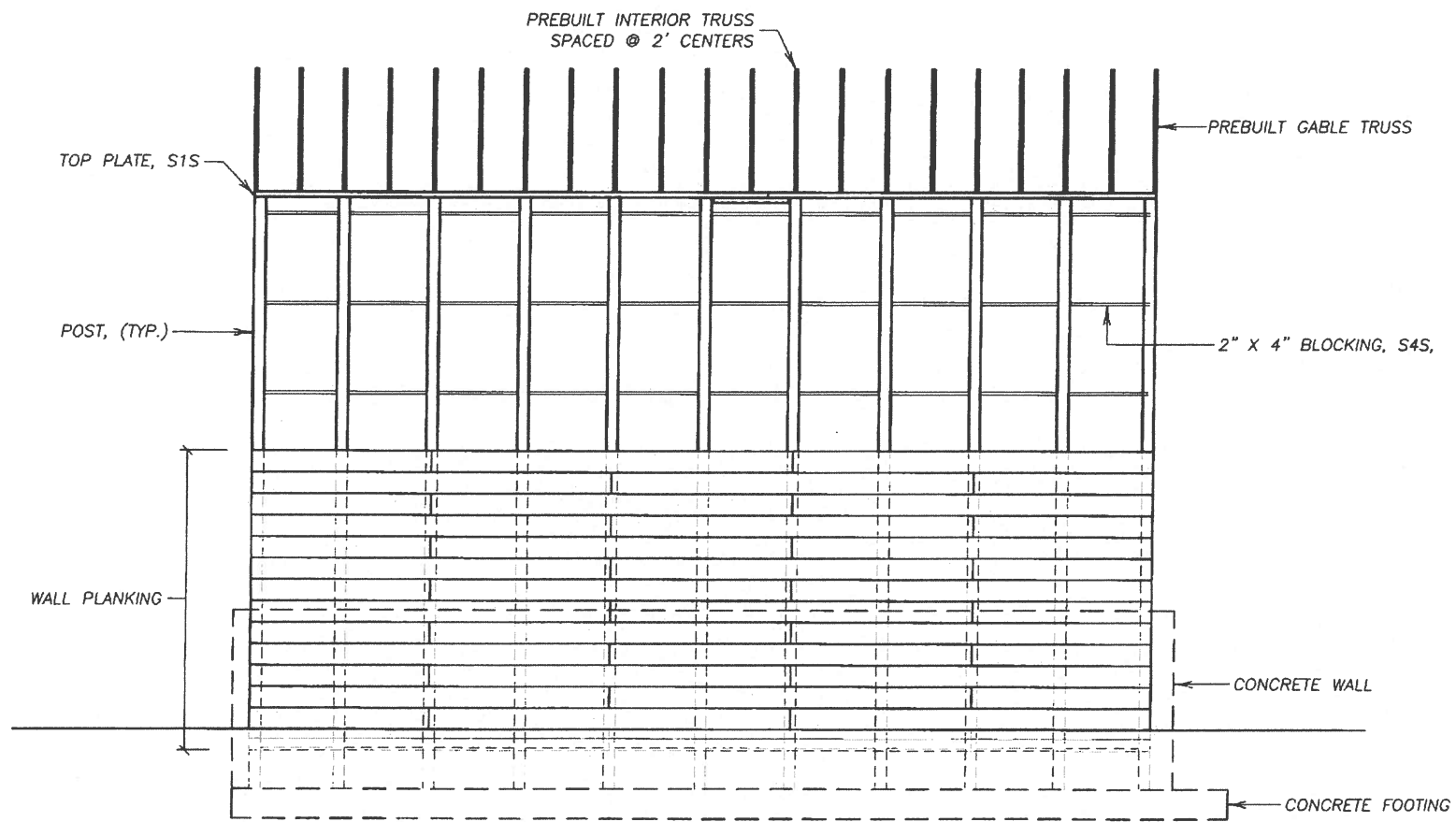
SIDEWALL FRAMING VIEWING FROM INSIDE STRUCTURE
