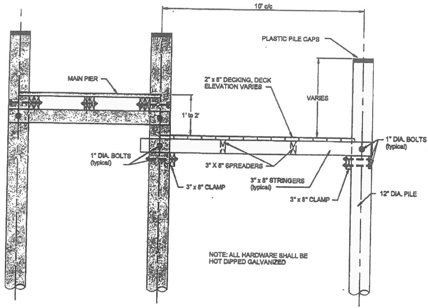
ELEVATION VIEW
